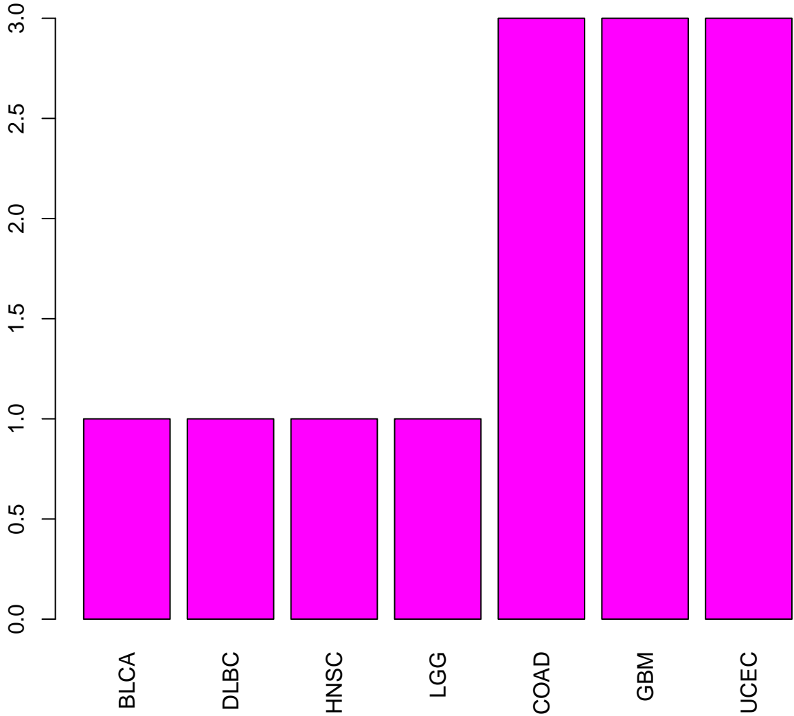
Total number of PTEN R335 mutations in different cancer types
