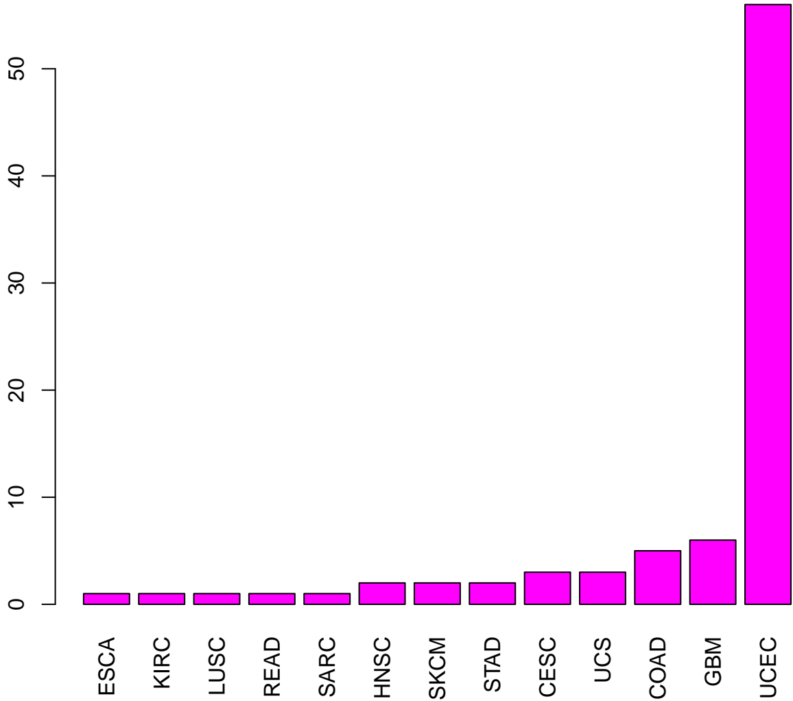
Total number of PTEN R130 mutations in different cancer types
