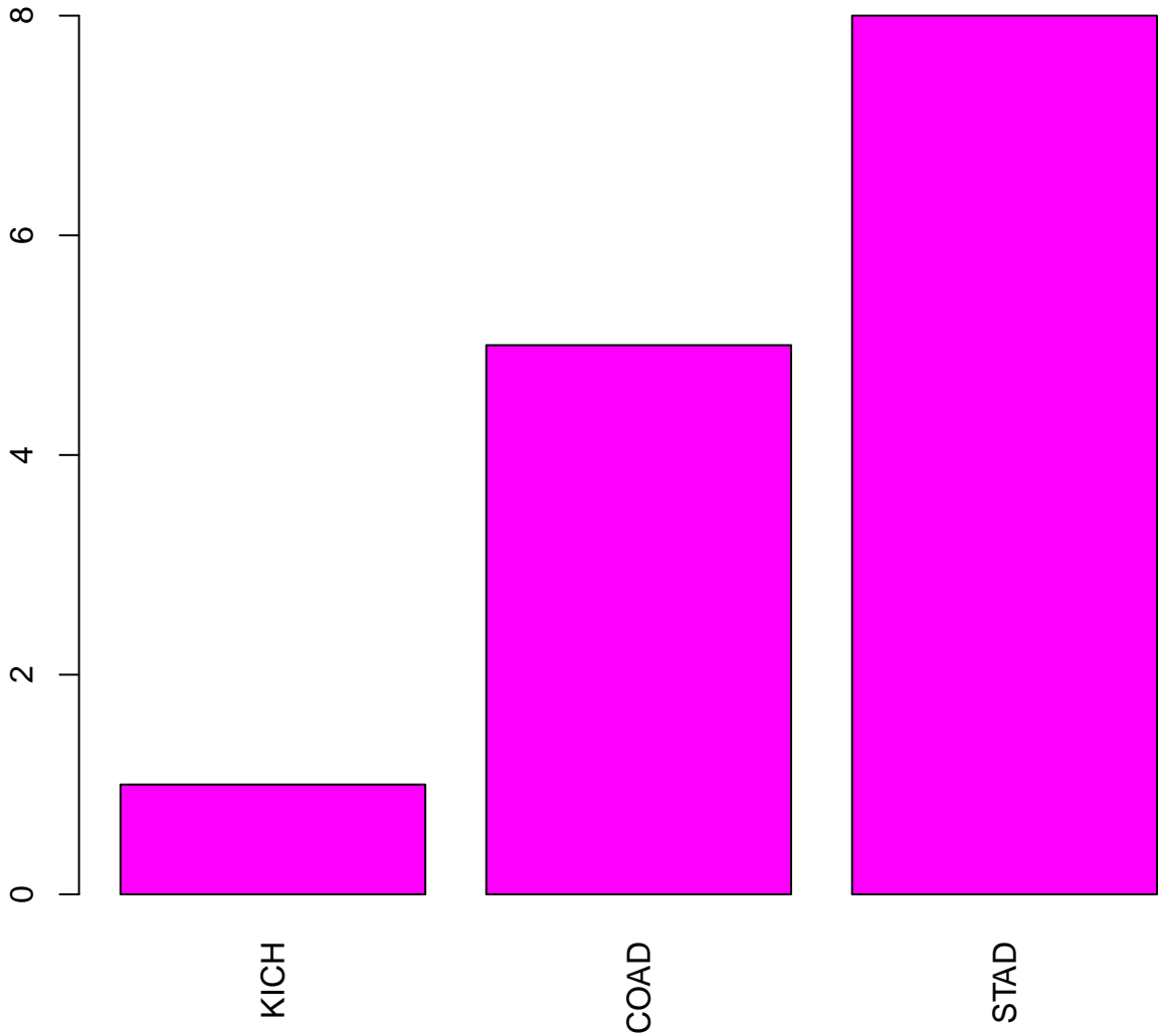
Total number of PTEN L265 mutations in different cancer types
