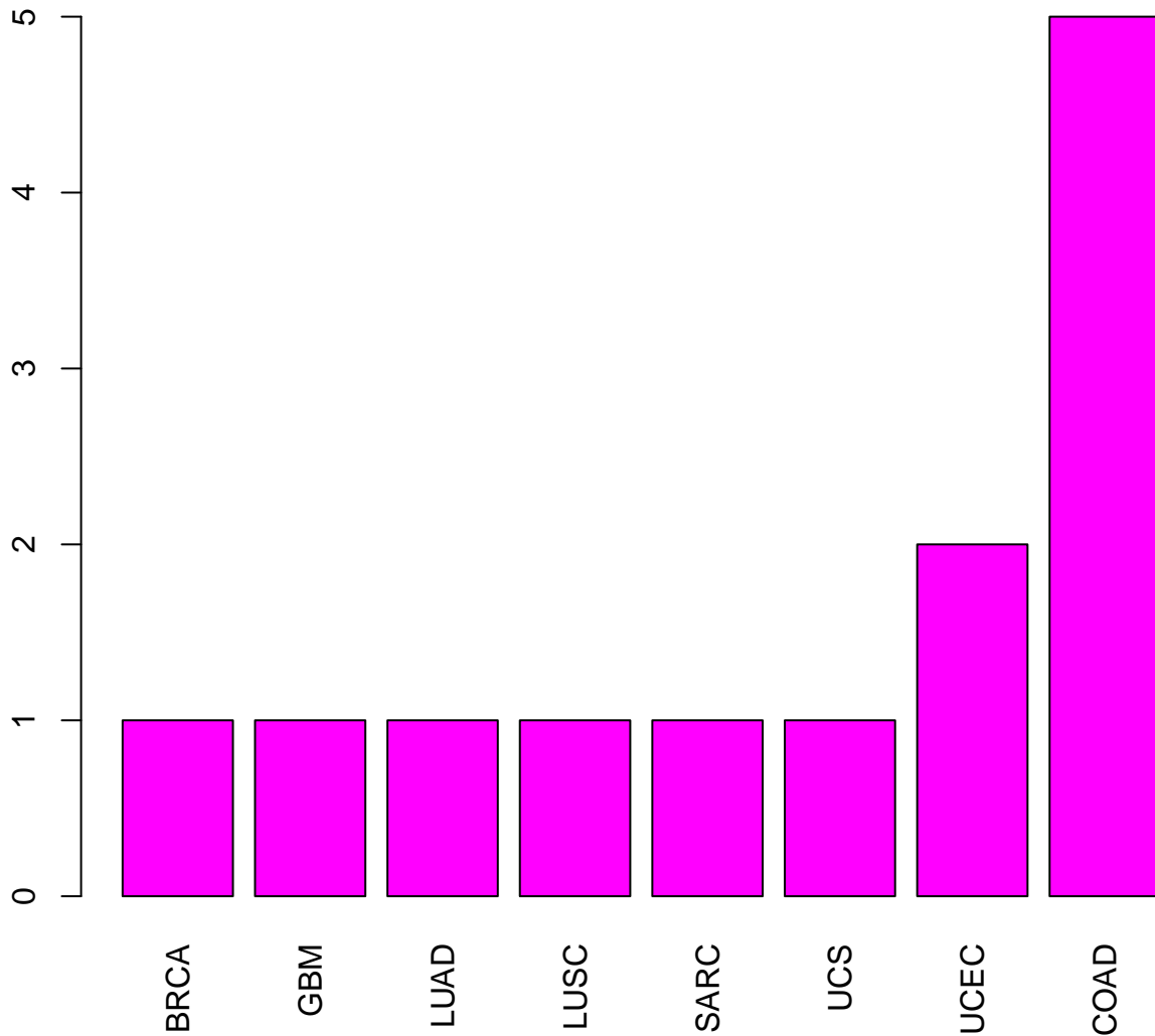
Total number of PTEN D92 mutations in different cancer types
