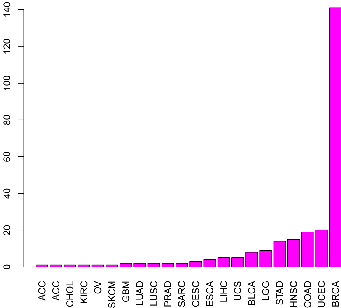
Total number of PIK3CA H1047 mutations in different cancer types
