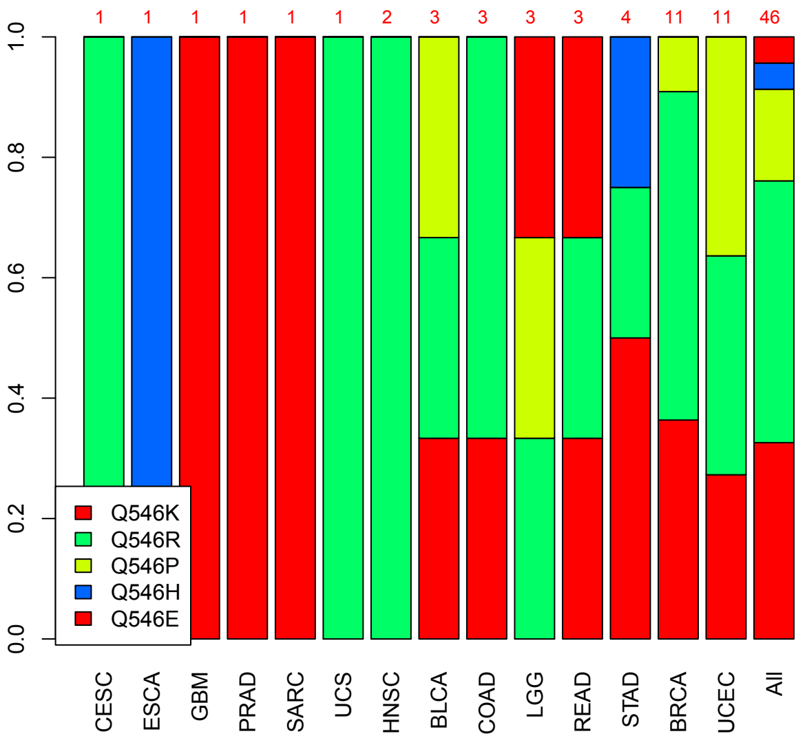
Proportional view of allele breakdown of PIK3CA Q546 mutations
